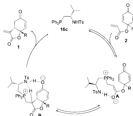
Scheme 2. Proposed mechanism of the RC reaction.
