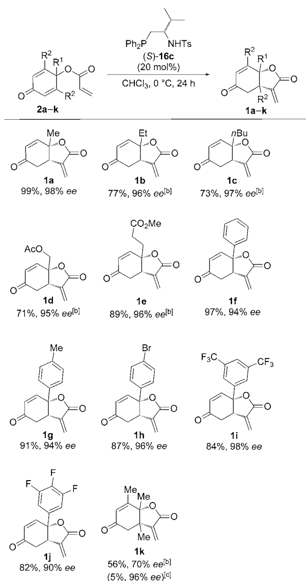
Scheme 1. Scope of the enantioselective RC reaction. Yields of isolated 1 . The ee values of 1 were determined by HPLC (Daicel Chiralpak IA, IB, IC, AD or AD3). [b] Reaction conditions: (S)- 16c (30 mol%), CHCl 3 , 0 °C, 72 h. [c] Phenol (50 mol%) was used with the optimized reaction conditions.
