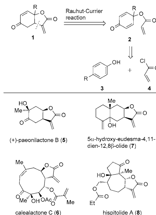
Figure 1. Retrosynthetic analysis of compound 1 and examples of \alpha -alkylidene- \gamma -butyrolactones isolated from natural sources.
